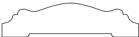
4144 .625 x 2.500
