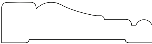
105 .750 x 2.750
