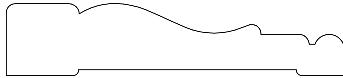
106 .750 x 3.500
